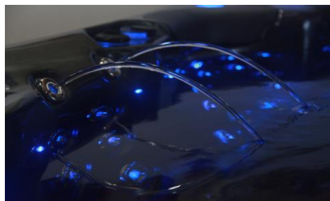
Laminar jets
